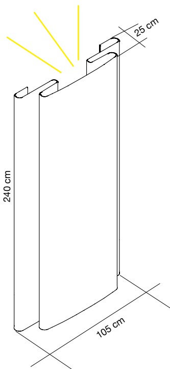
Snowsound-Fiber 6,5 m 2
